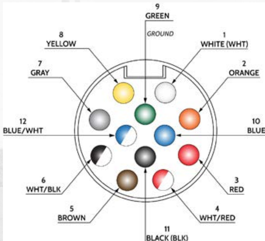
Figure 8 - HD Detector Cable Wire Colors
