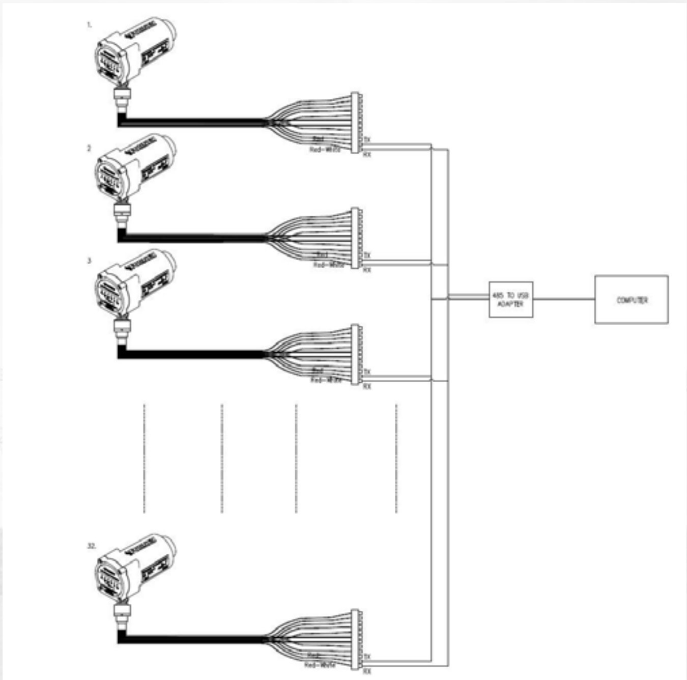
Figure 10 – Daisy Chain for HD Flame Detectors
