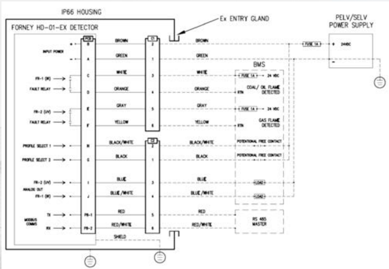
Figure 9 - Wiring Diagram
