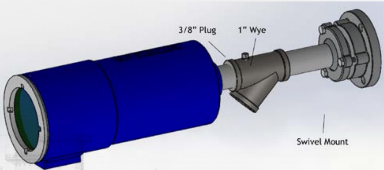
Figure 7 - Swivel Mount, Wye and Detector Assembly
