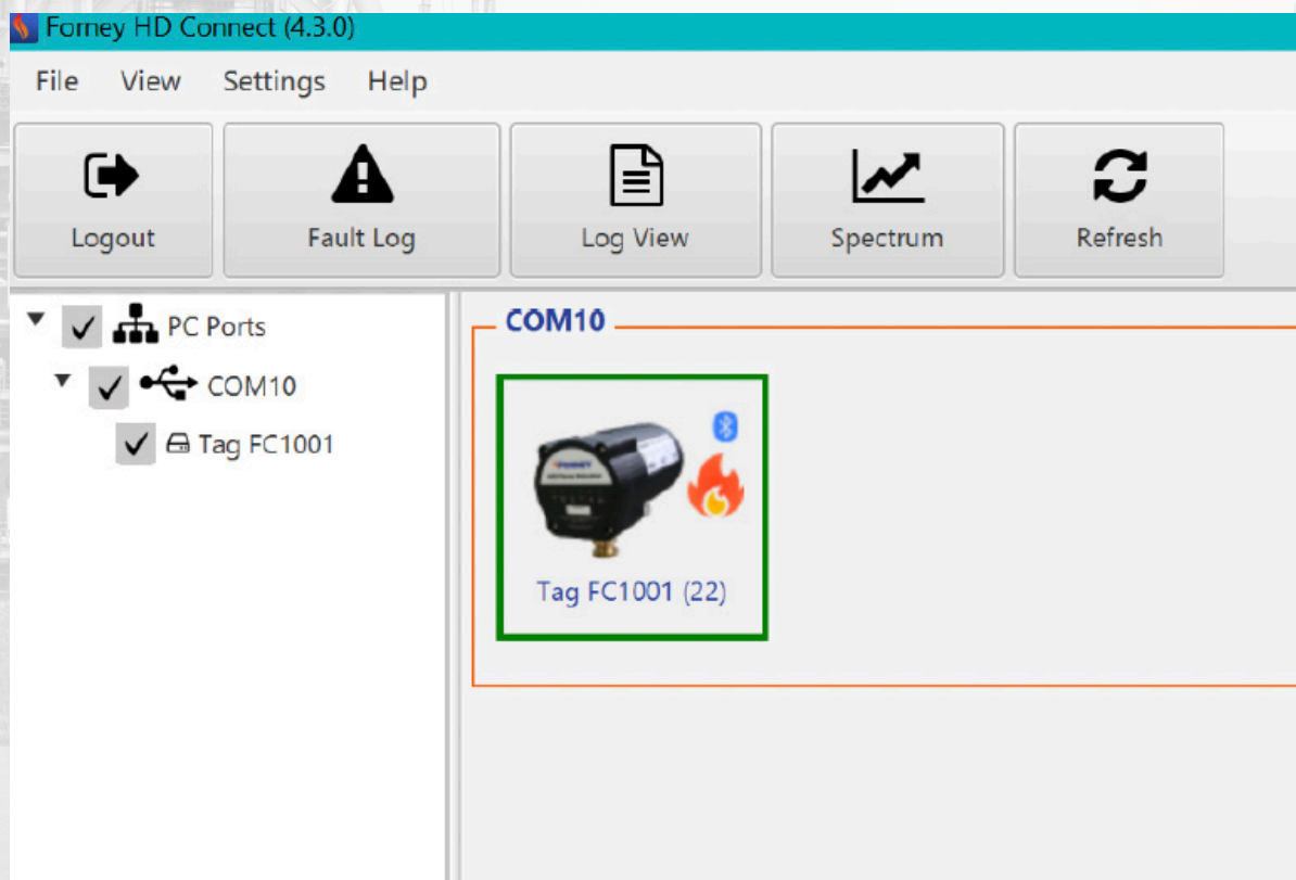
Figure 4 Welcome Screen
