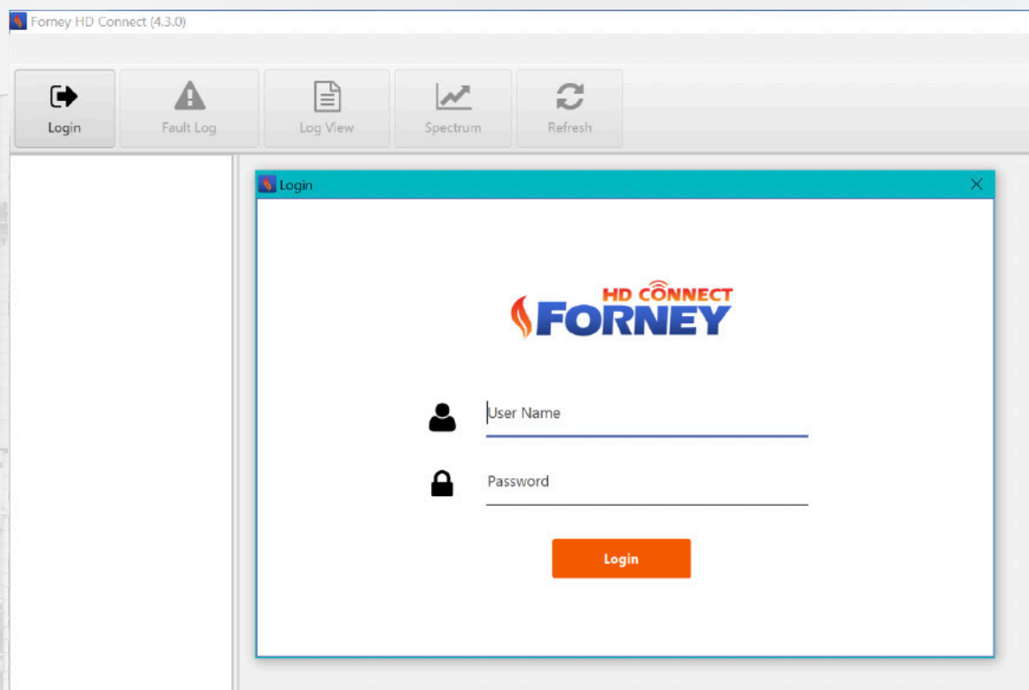
Figure 1 Login Screen
