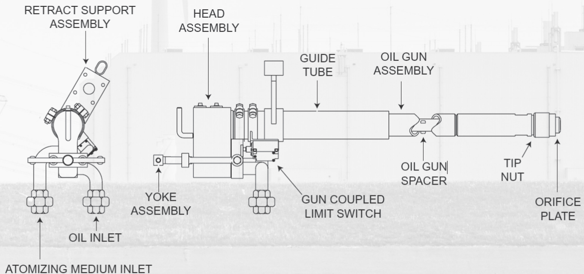
(RIGID DESIGN SHOWN WITHOUT RETRACT ASSEMBLY)
