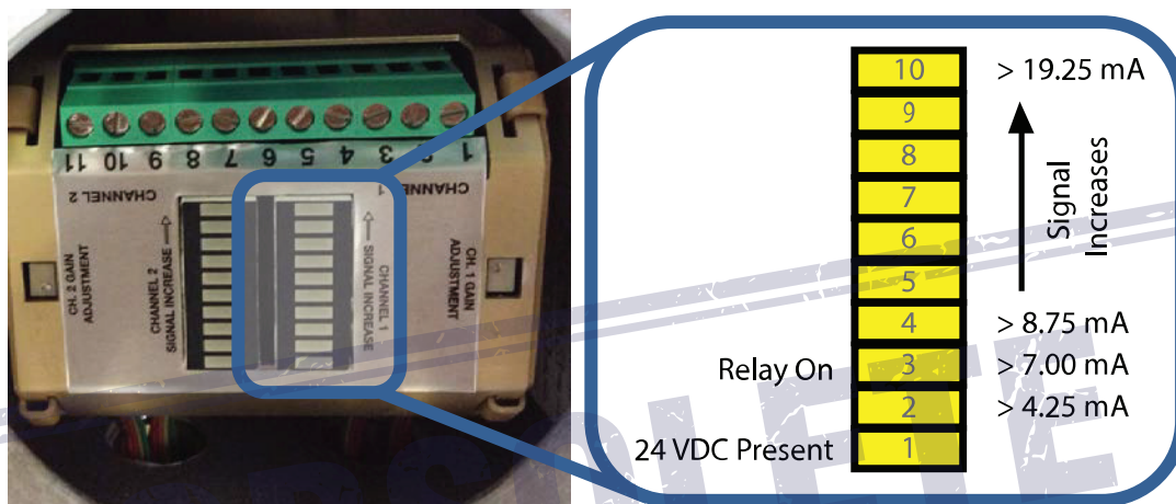
Figure 8 LED Indicators
