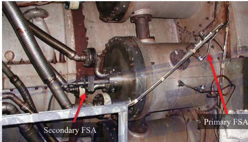
Figure 4 Frame Engine Primary and Secondary Installations
