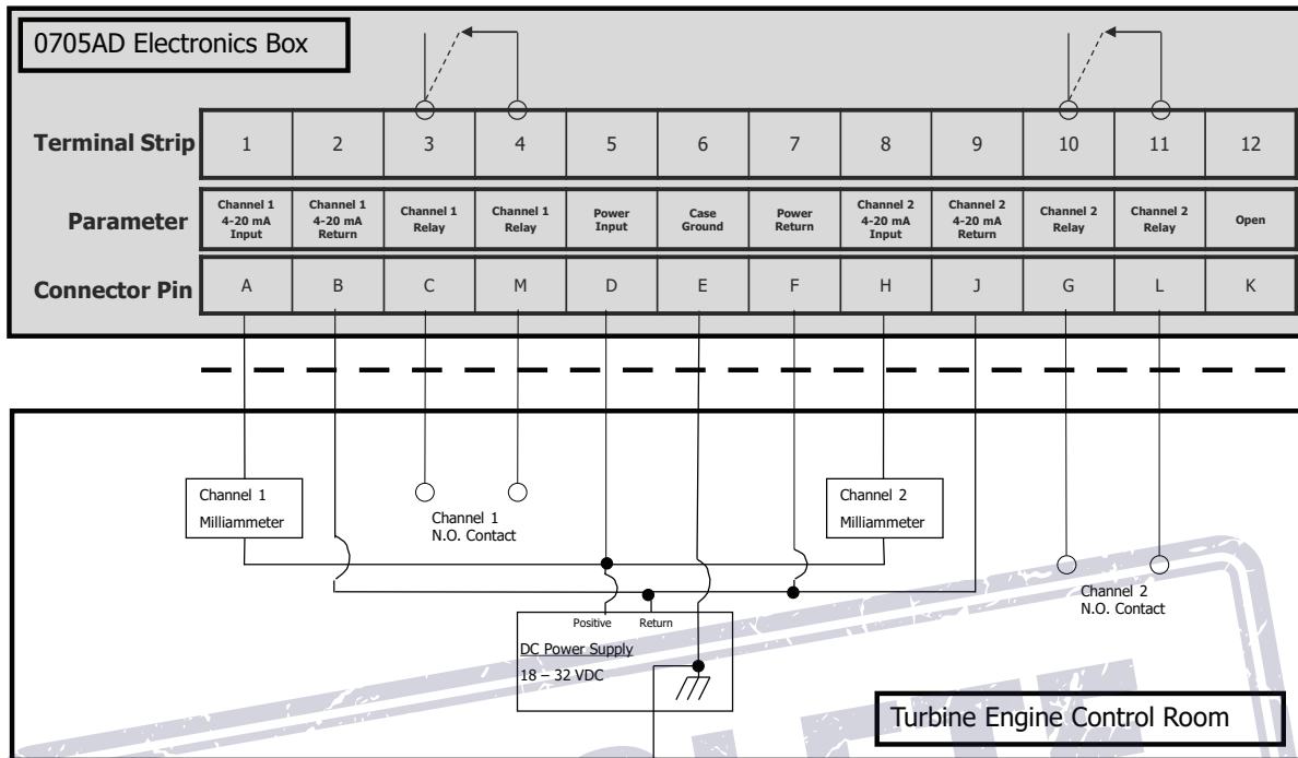
Figure 14 Simultaneous 4-20mA and Relay Operation Diagram
