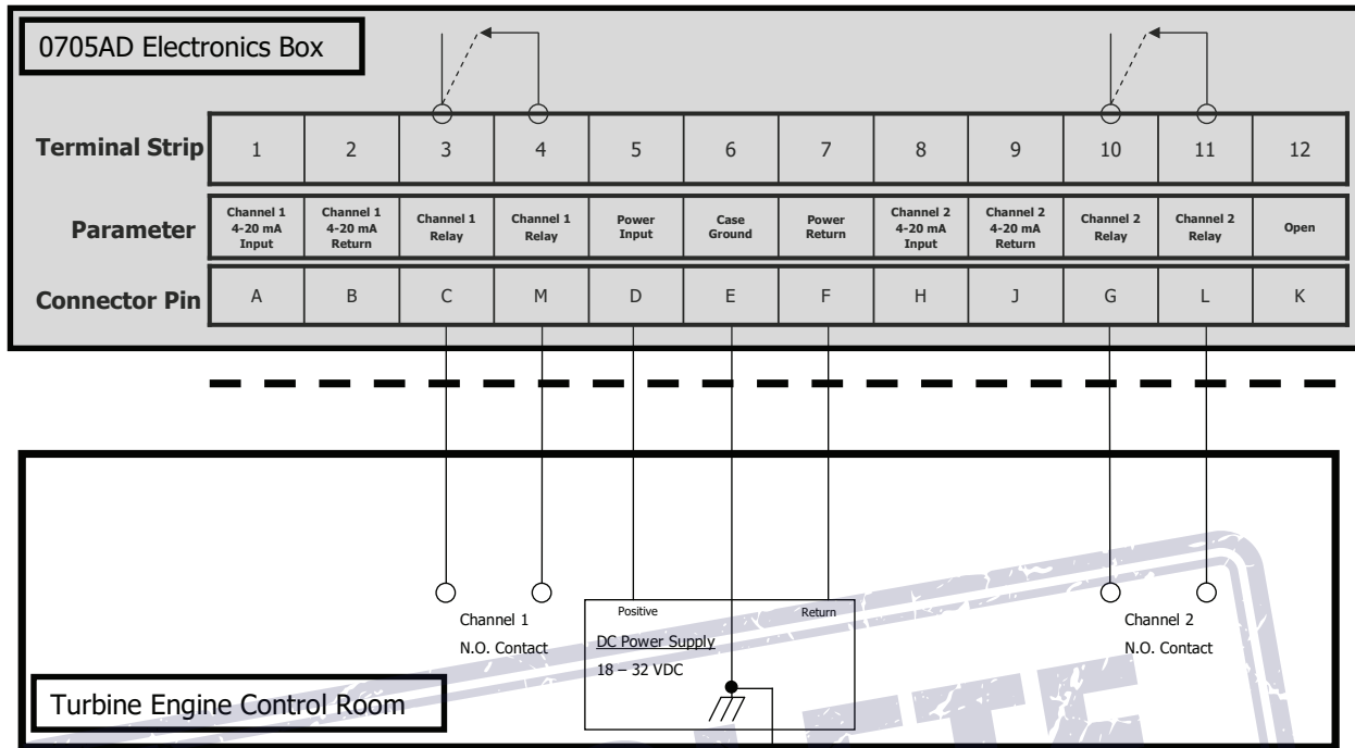
Figure 13 Configuration for Relay Output
