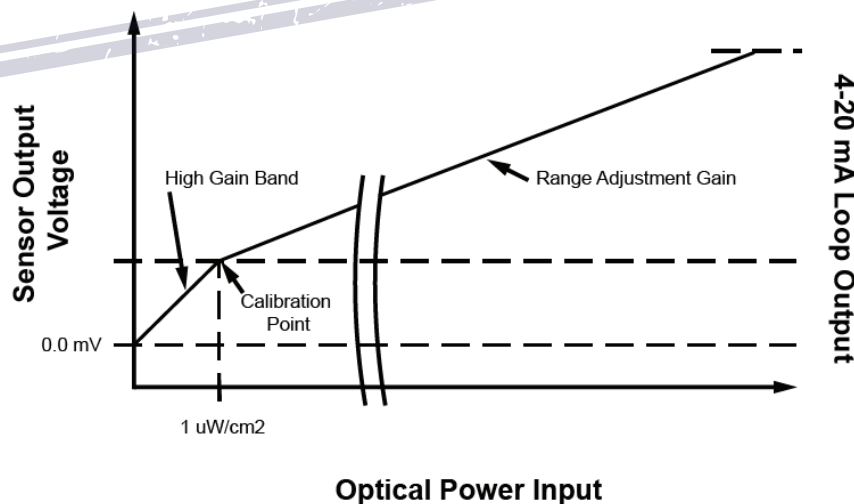
Figure 9 Plot of current output vs. light energy input
