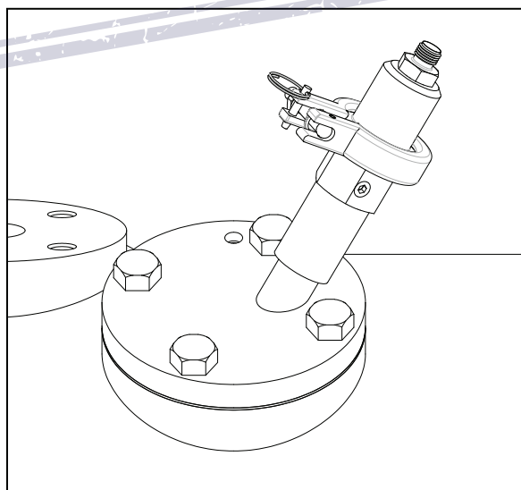
Figure 10 GE Frame Engine FSA, Typical Primary Zone Installation
