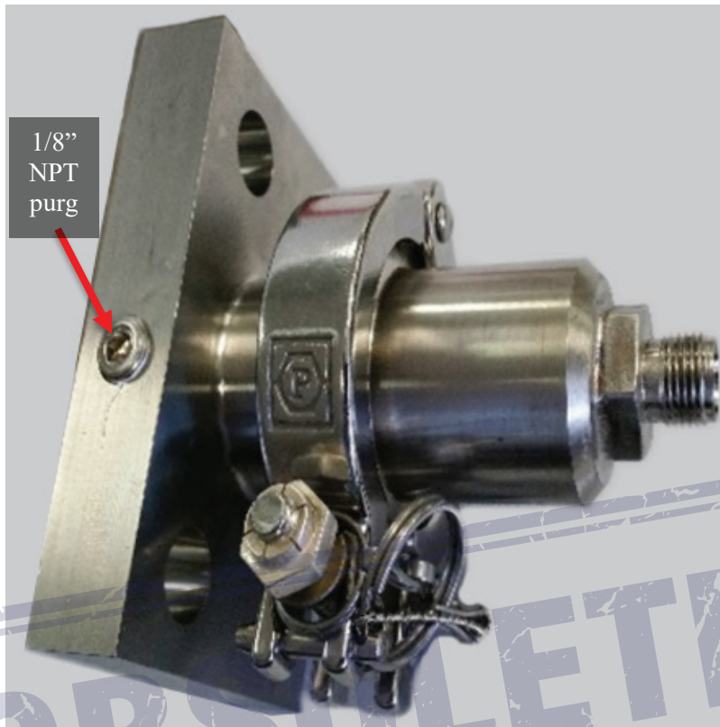
Figure 6 Frame Engine FSA Flange Design
